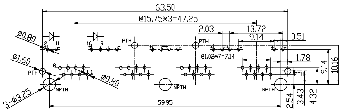
PC BOARD LAYOUT THICKNESS=1.6mm
